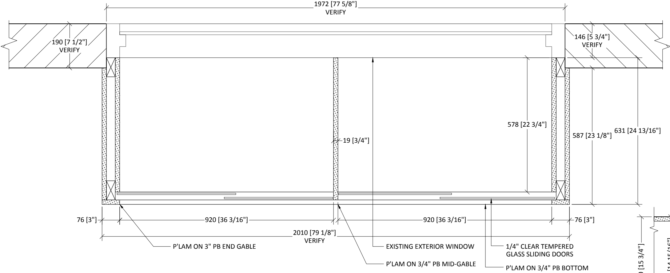
U ROOM 114A - SCIENCE LAB - SECTION ARCH. REF.: 2/A8.3 Scale: 1:10
