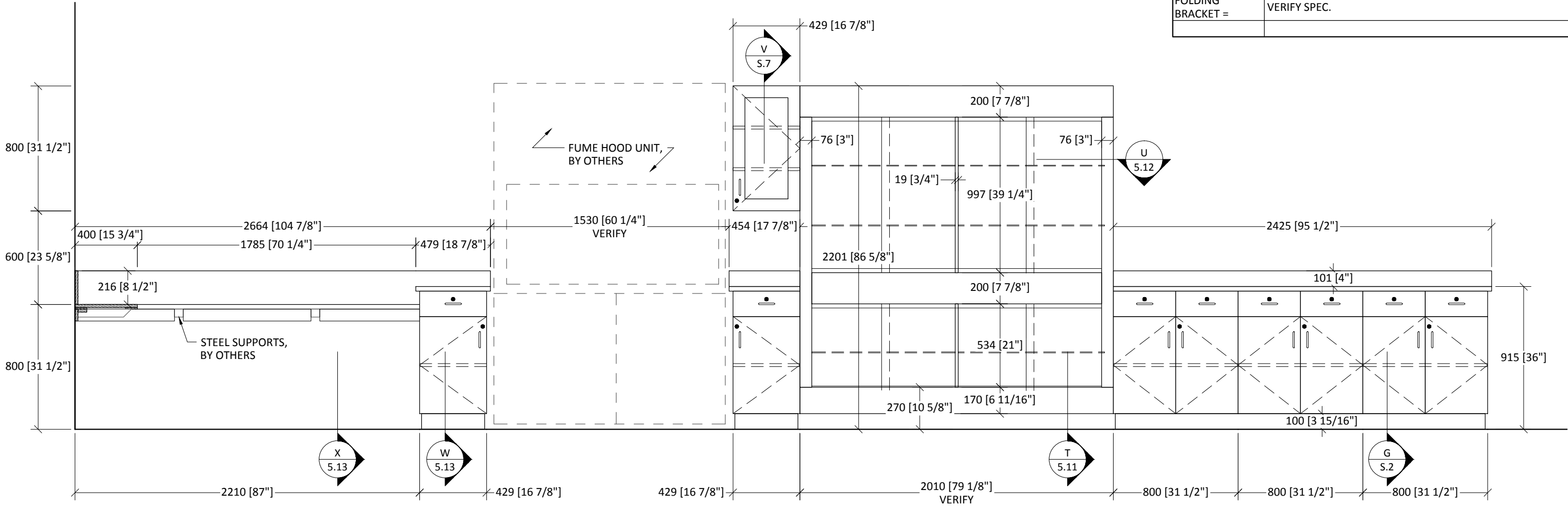
B ROOM 114A - SCIENCE LAB - ELEVATION ARCH. REF.: 2/A7.3 Scale: 1:20
