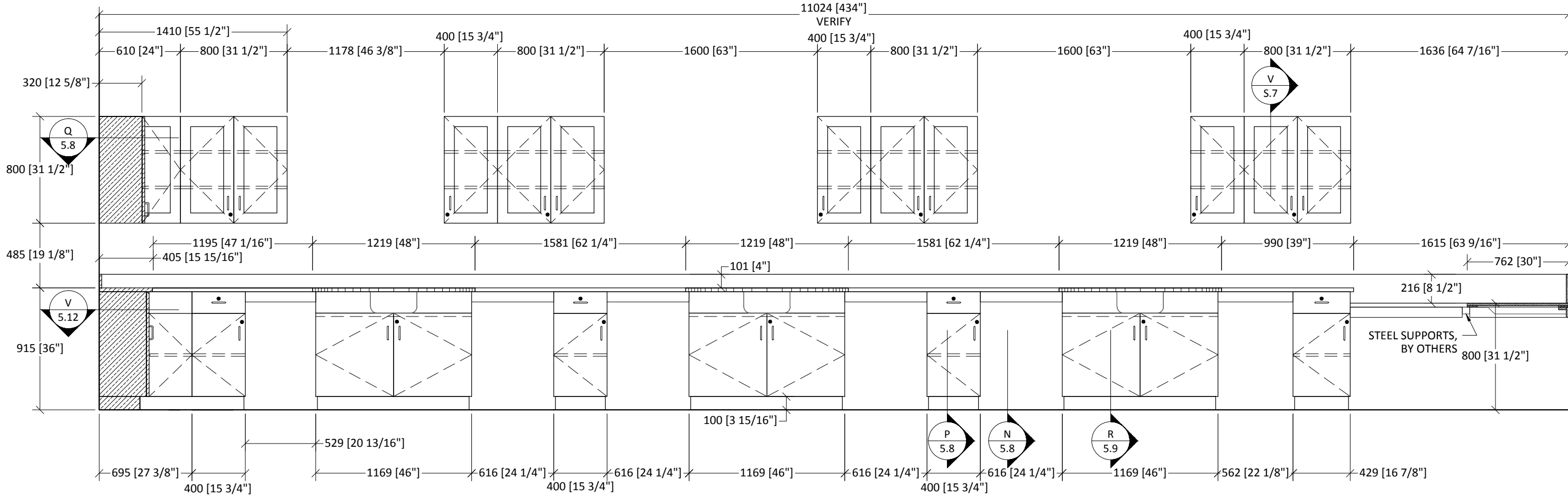
E ROOM 114A - SCIENCE LAB - ELEVATION ARCH. REF.: 3/A7.3 Scale: 1:30
