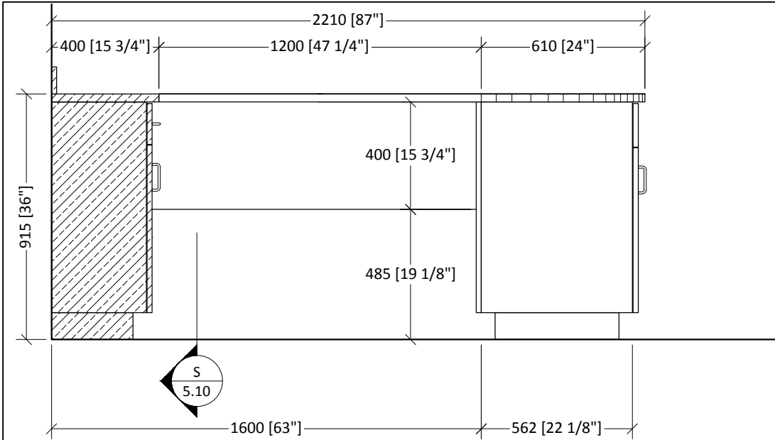
C ROOM 114A - SCIENCE LAB - ELEVATION ARCH. REF.: 10/A7.3 Scale: 1:30
