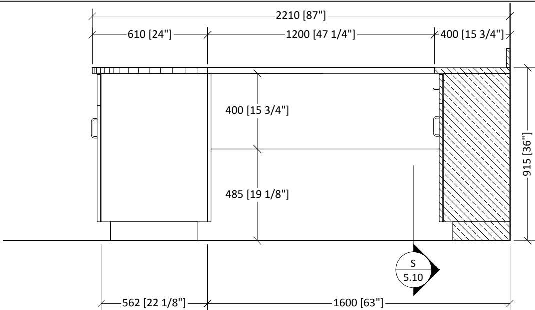
D ROOM 114A - SCIENCE LAB - ELEVATION ARCH. REF.: 10/A7.3 Scale: 1:30
