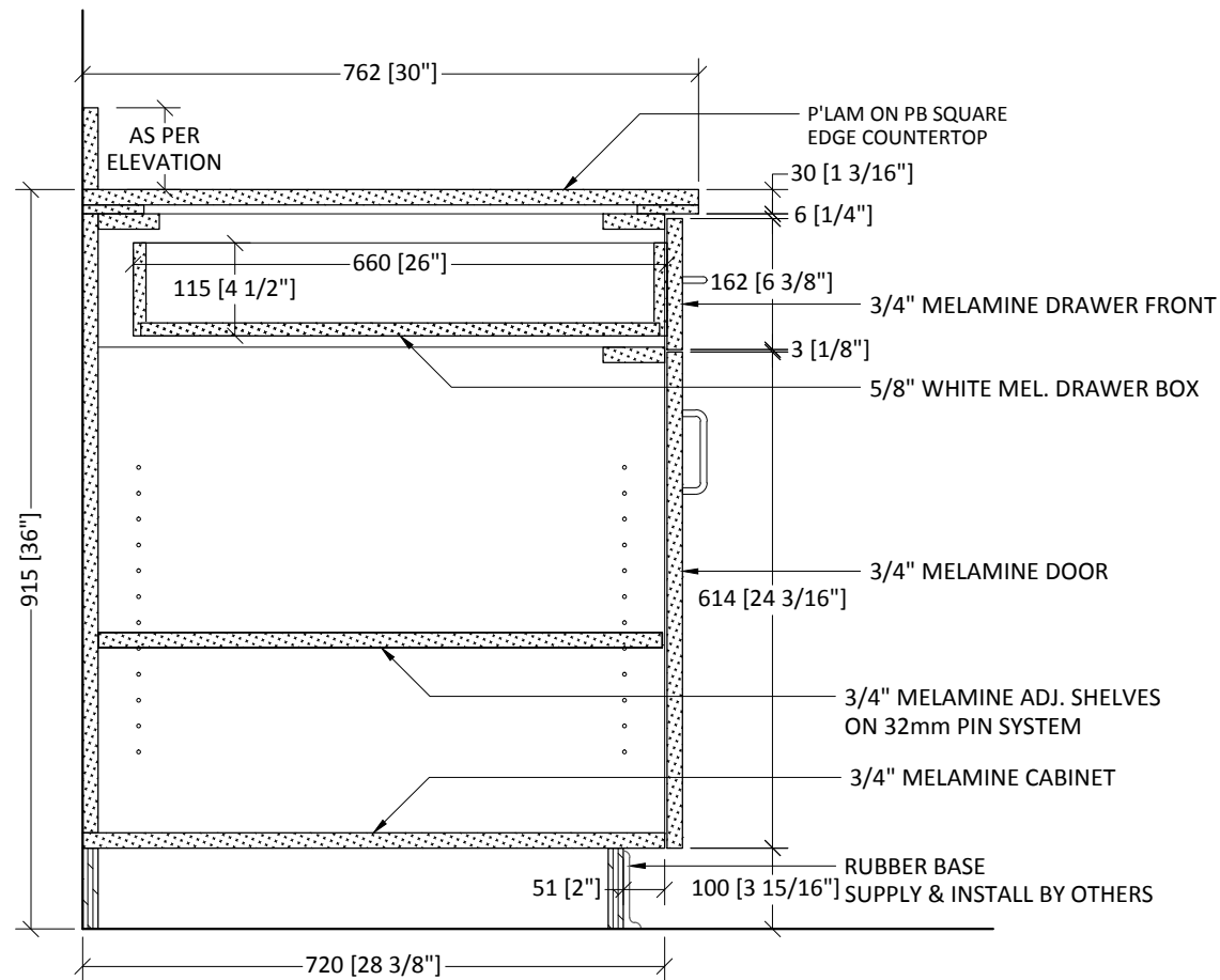
W DOOR/DRAWER CABINET - SECTION 1/A8.1 SIM. Scale: 1:10
