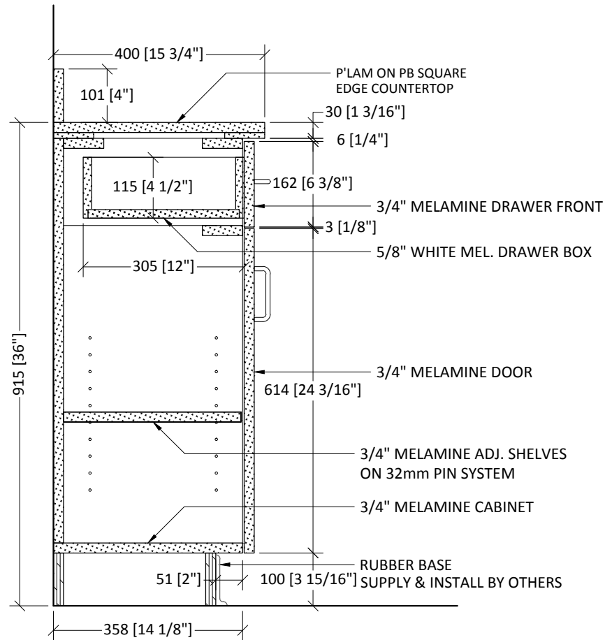
P ROOM 114A - SCIENCE LAB - SECTION ARCH. REF.: 1/A8.1 Scale: 1:10
