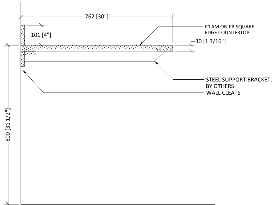
X DOOR/DRAWER CABINET - SECTION 1/A8.1 Scale: 1:10
